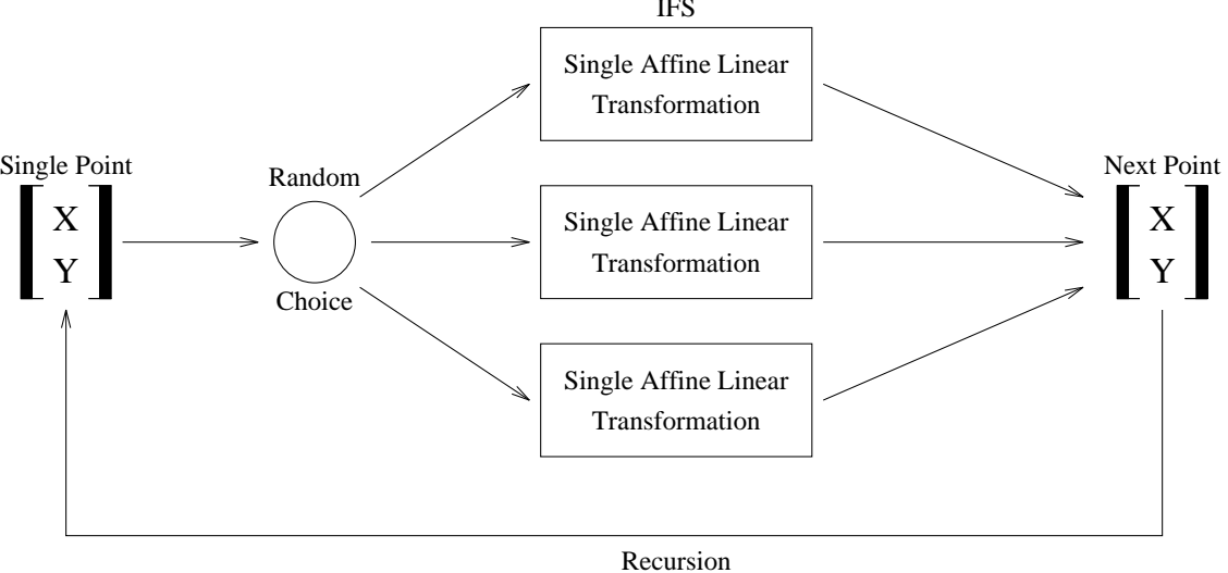
Figure 7.8 A schematic of the IFS algorithm: A single point is transformed by a single randomly chosen transformation.
