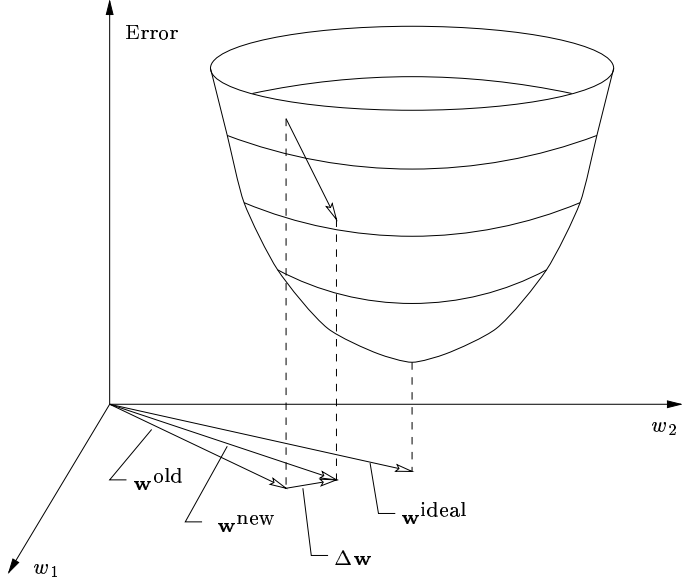
Figure 22.3 The delta rule as a steepest descent step in the error surface. Figure adapted from (Caudill & Butler, 1990).
