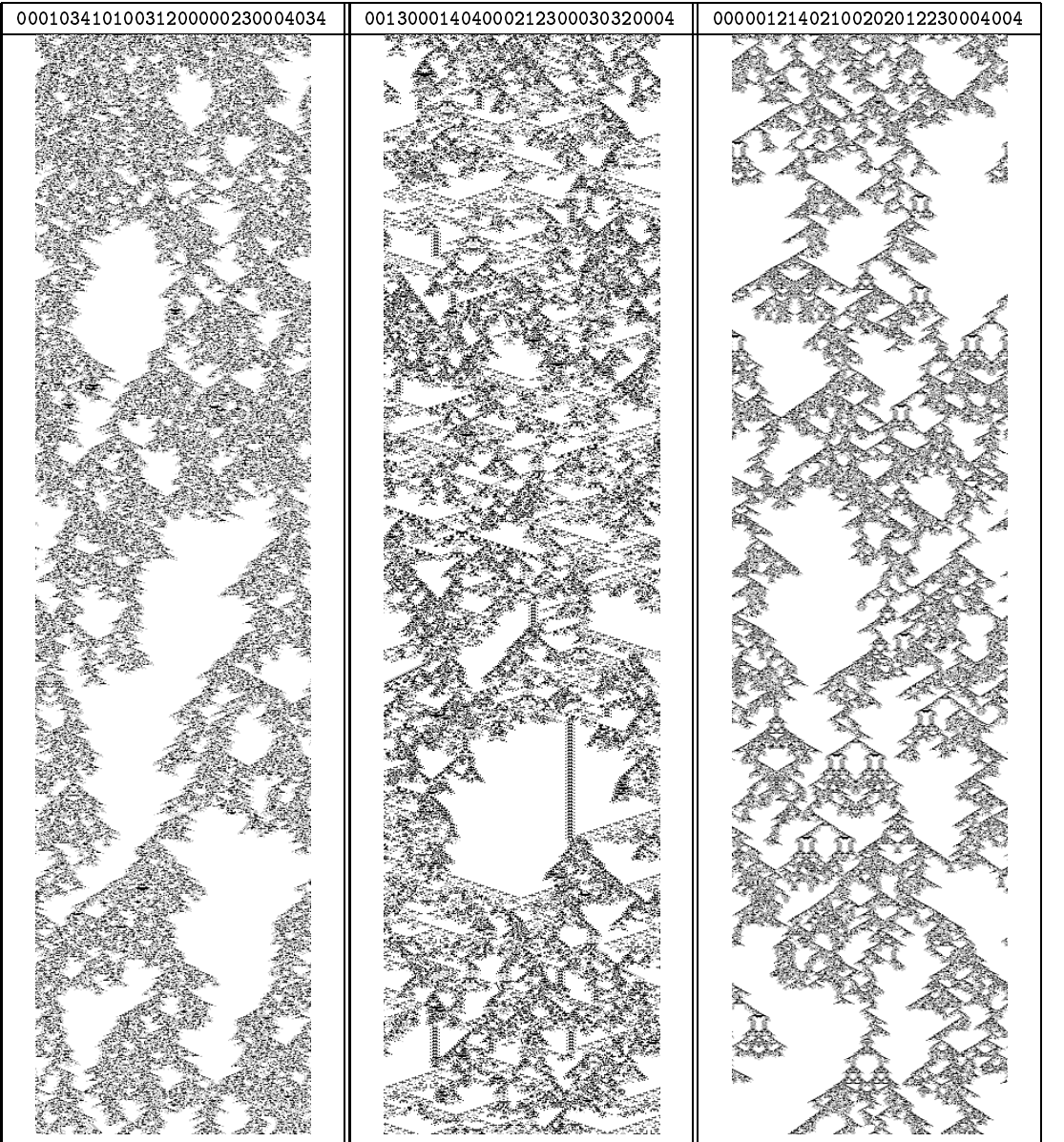
Figure 15.8 Examples of Wolfram's Class IV
